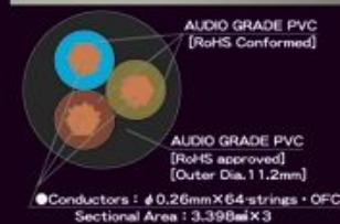
G.S.#302 nano3 Sectional Drawing
