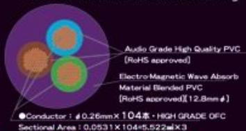
#307 EXTREME Sectional Drawing
